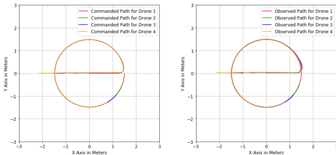
(a) Commanded positions for a platoon of four drones with a formation distance parameter (FDP) of 0.50 meters in waypoint following mode.
