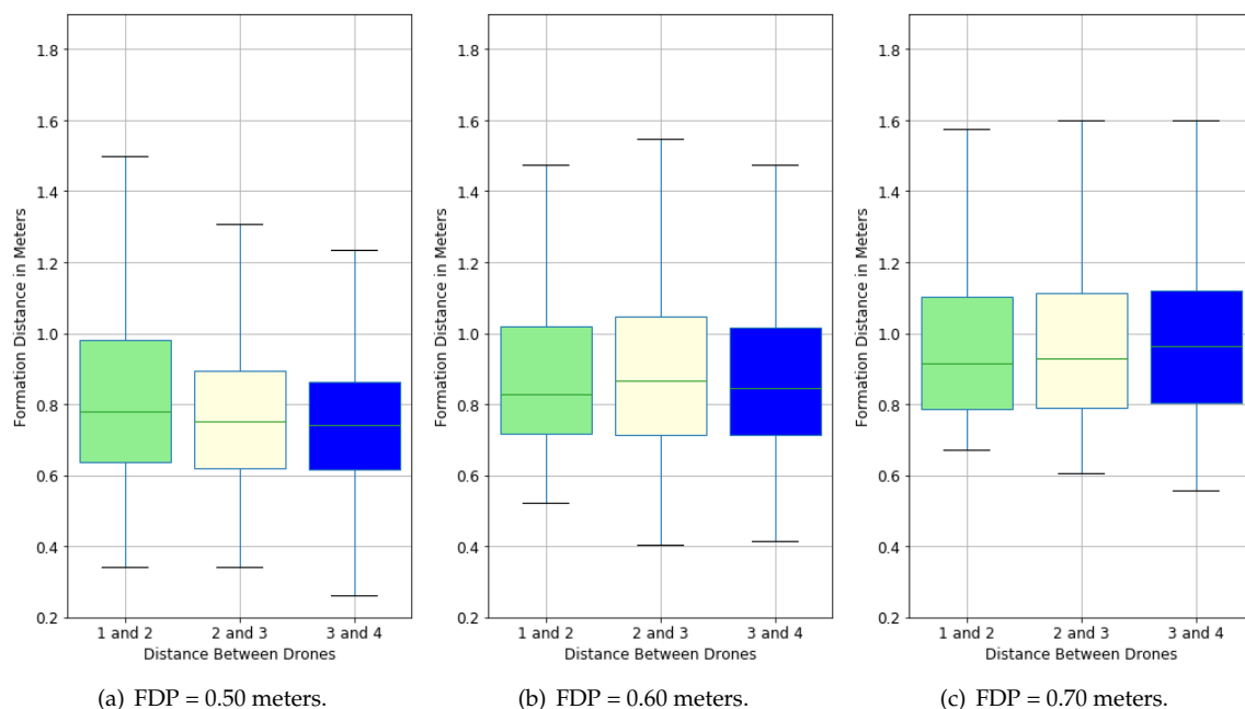
Figure 13. Observed path boxplots for different formation distance parameters (FDP) with a box size of 0.20 meters.
