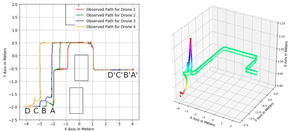
(a) Observed pathfinding paths of a four drone platoon. Starting from the positions A to D and ending on positions A' to D'. Obstacles depicted as rectangles.
