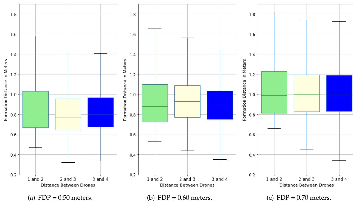
Figure 14. Observed path boxplots for different formation distance parameters (FDP) with a box size of 0.25 meters.
