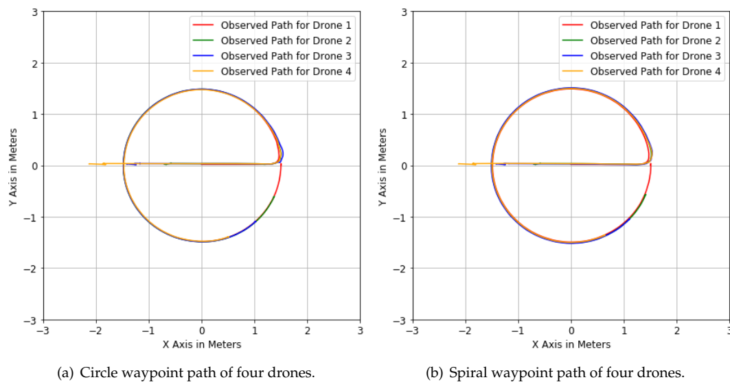
Figure 9. Comparison between observed circle and spiral waypoint paths for a formation distance parameter (FDP) of 0.60 meters, both depicted from above, i.e., on the x - y coordinate level.
