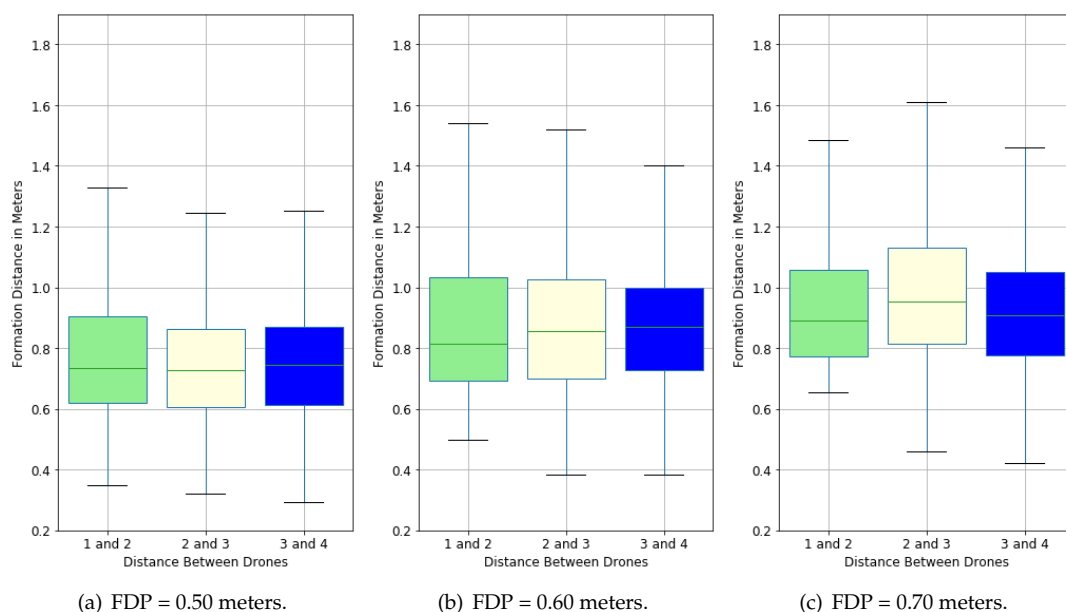
Figure 12. Observed path boxplots for different formation distance parameters (FDP) with a box size of 0.15 meters.
