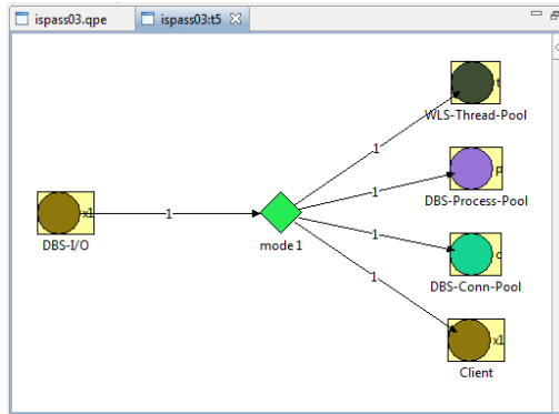
Fig. 2. QPE Incidence Function Editor
