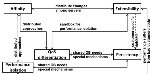
Figure 2: Interdependencies between different architectural concerns.
