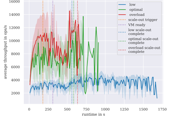
Fig. 6: Couchbase—elastic scale-out, read-heavy workload
