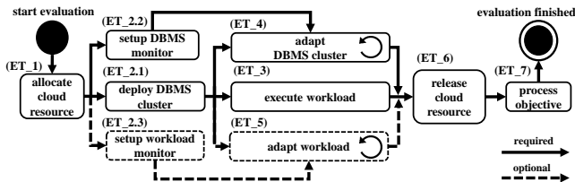
Fig. 2: Elasticity Evaluation Process
