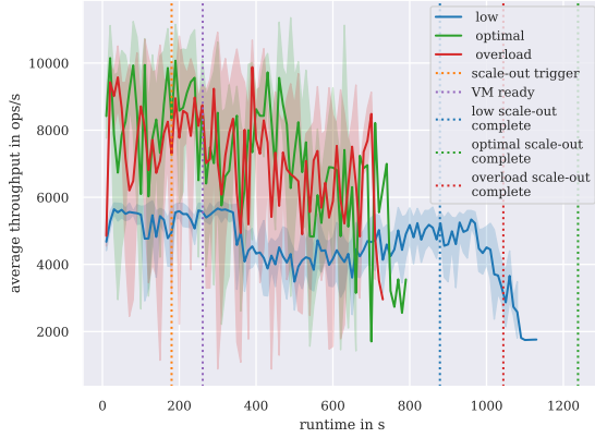
Fig. 8: Couchbase—elastic scale-out, write-heavy workload
