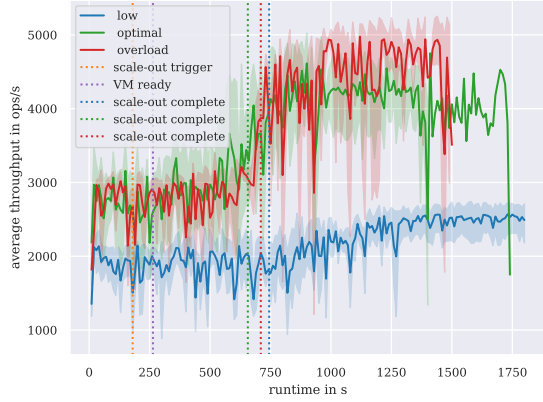
Fig. 5: Cassandra—elastic scale-out, read-heavy workload
